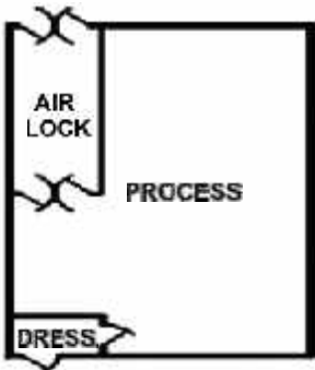
CLEAN ROOM 10,000 Class - Certified 26' x 50' x 14' High Manufacturing Facility
